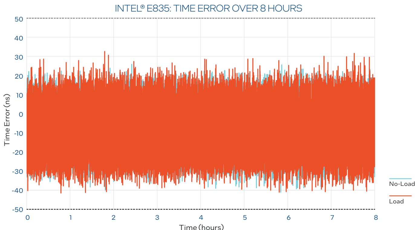
Figure B-1: Intel® E835-XXVDA2 error rates over 8-hr test (Source: Signal65).
