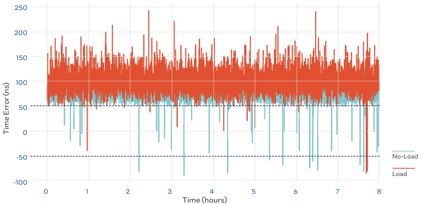
Figure B-3: NVIDIA® CX7 error rates over 8-hr test (Source: Signal65).
