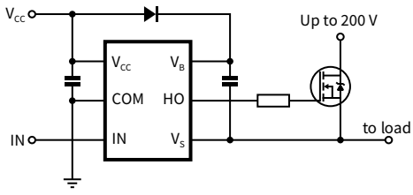
Typical connection
