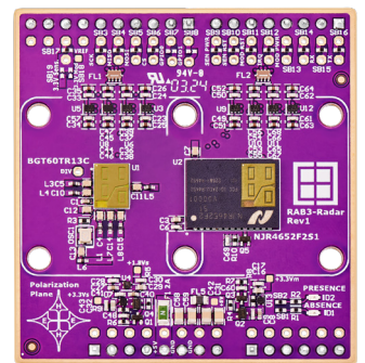
Radar Board Module & Sensor RAB3
