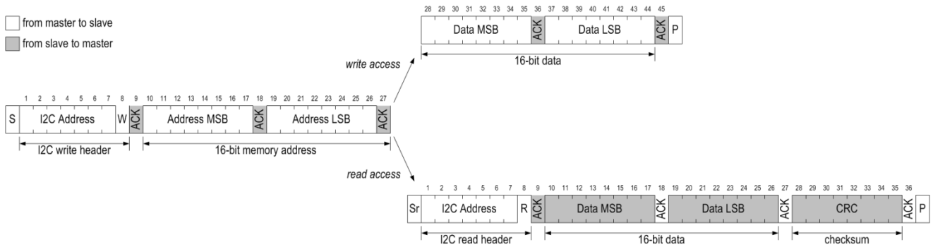
Figure 9 Communication sequence for starting a measurement and reading measurement results.
