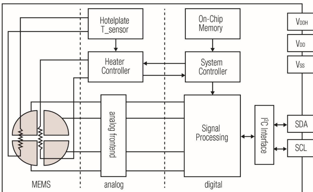
Figure 1 Functional block diagram of the SGP30.
