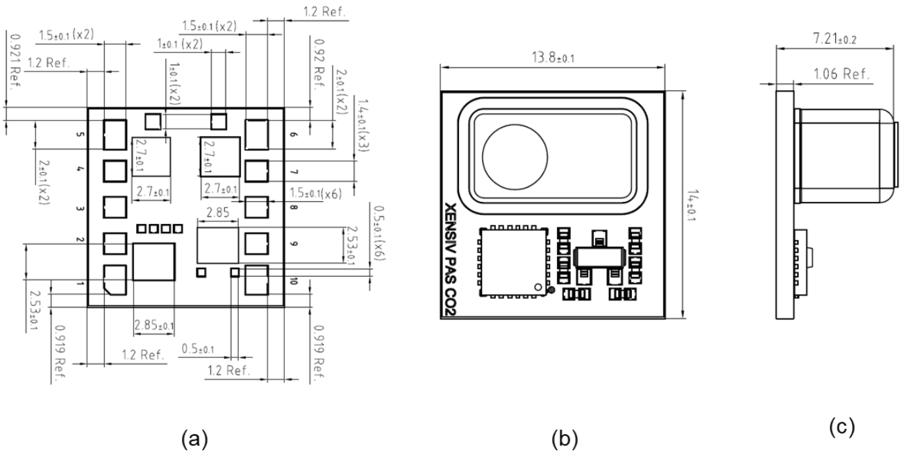
Figure 9 (a) Bottom view (b) Top view and (c) Side view. All dimensions are in mm.
