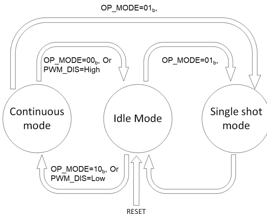
Figure 7 Operating mode transition
