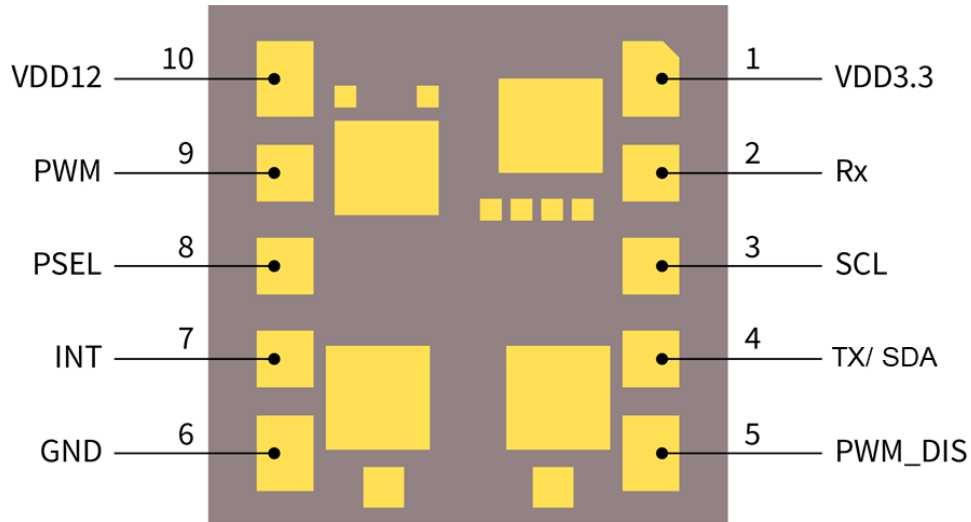
Figure 2 Pin-out diagram (Bottom view)
